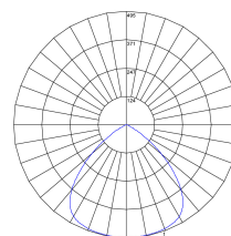
NOMINAL POLAR CURVE - DIRECT
