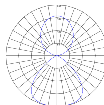
NOMINAL POLAR CURVE - DIRECT/INDIRECT
